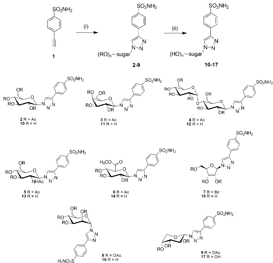
Scheme 2. Synthesis of Glycoconjugate Benzene Sulfonamide Library ( 2–17 ) from 1 and Sugar Panel a–h a
