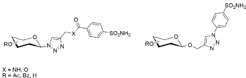
Figure 2. Generation I and II benzene sulfonamide glycoconjugates. 23–25
