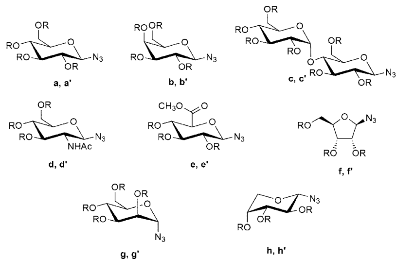
Figure 3. Azido sugar "tail" fragment panel: a–e, g, h ( R = \text{Ac} ); f ( R = \text{Bz} ); and a'–h' ( R = \text{H} ).
