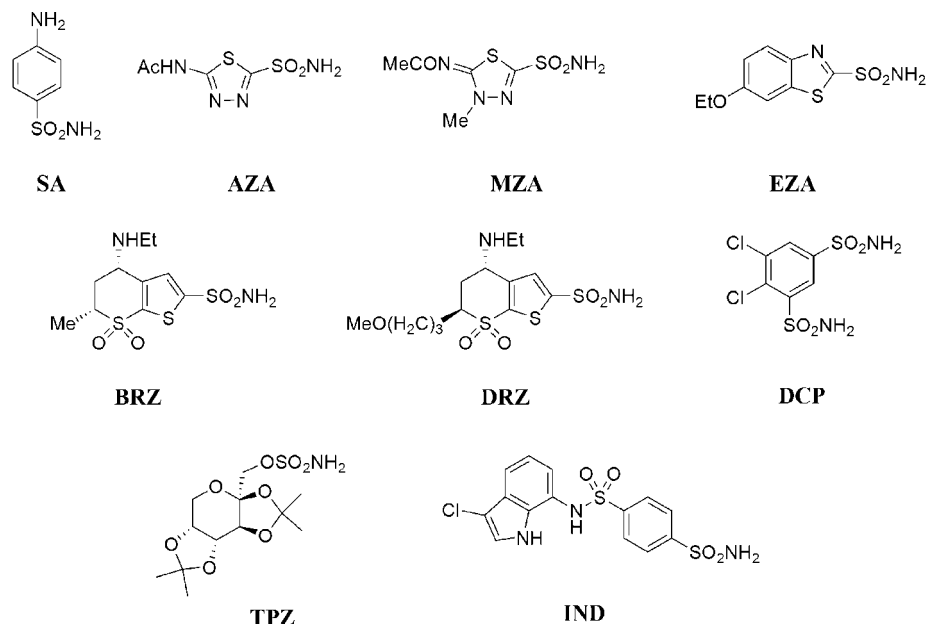
Figure 1. Known human CA inhibitors including some clinically used drugs.
